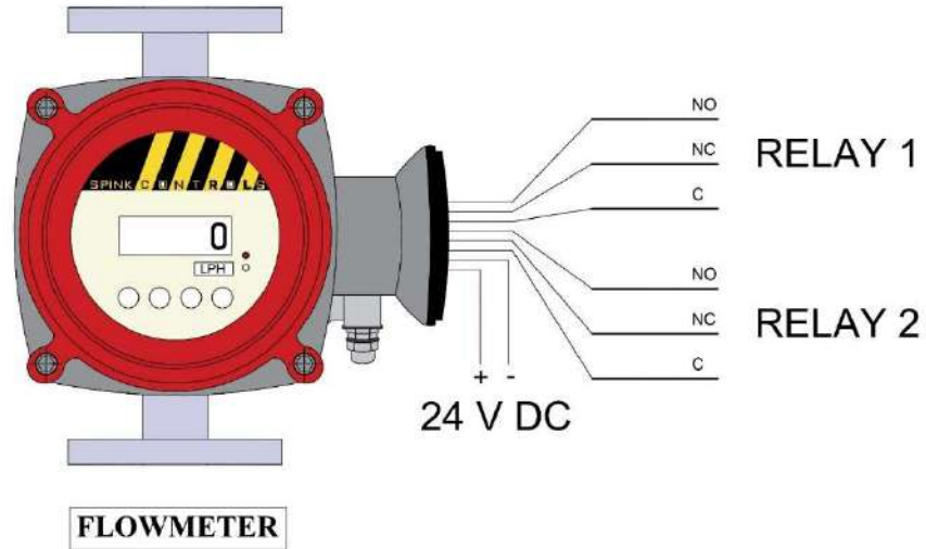
Fig No.: 5.2 – Electrical Connection for 24 V DC power supply
